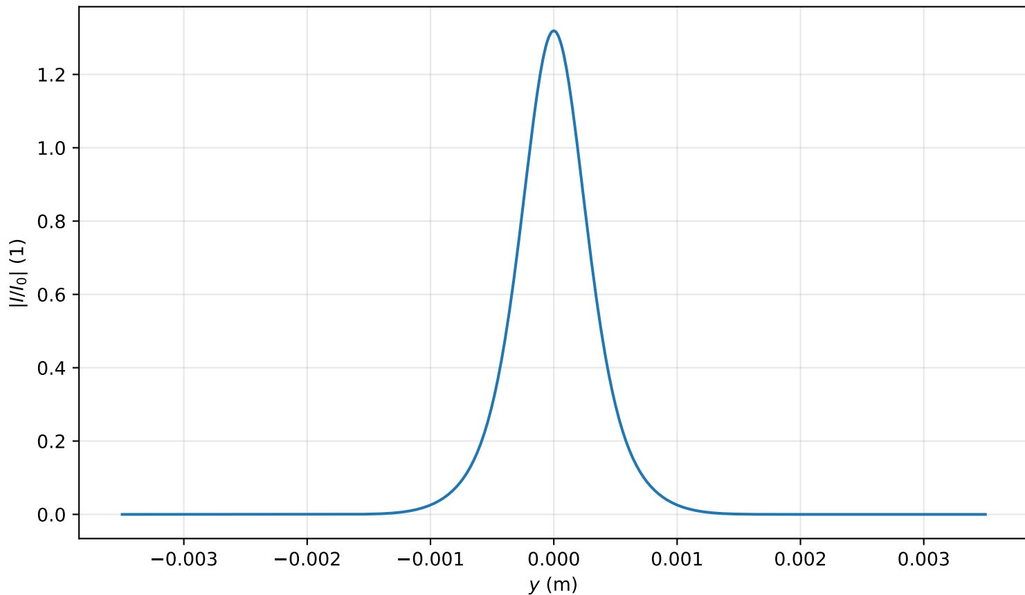
Intensity profile I(x=0, y, z=1.115)/I_0 , P_{in}=0.8P_{cr} , artificial time
